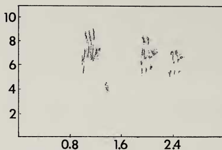
FIG. 4. Spectrograms of flight calls of Stephen's Lorikeet ( Vini stephensi ).
